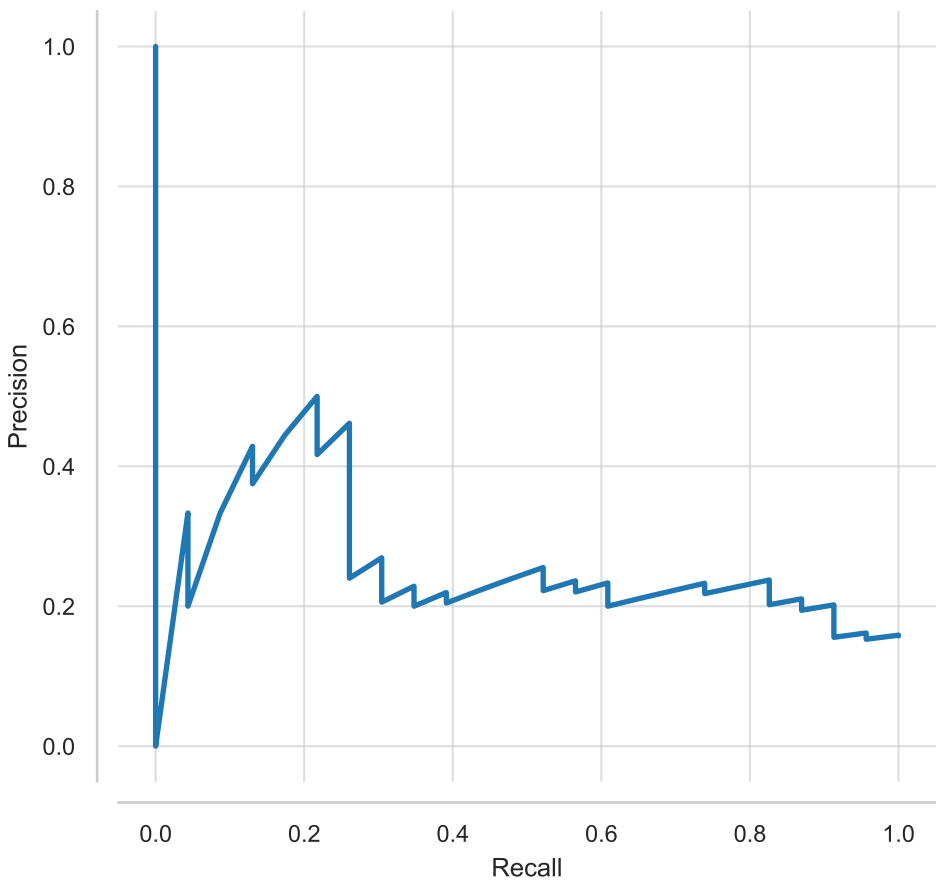
Precision-Recall Curve - LR
